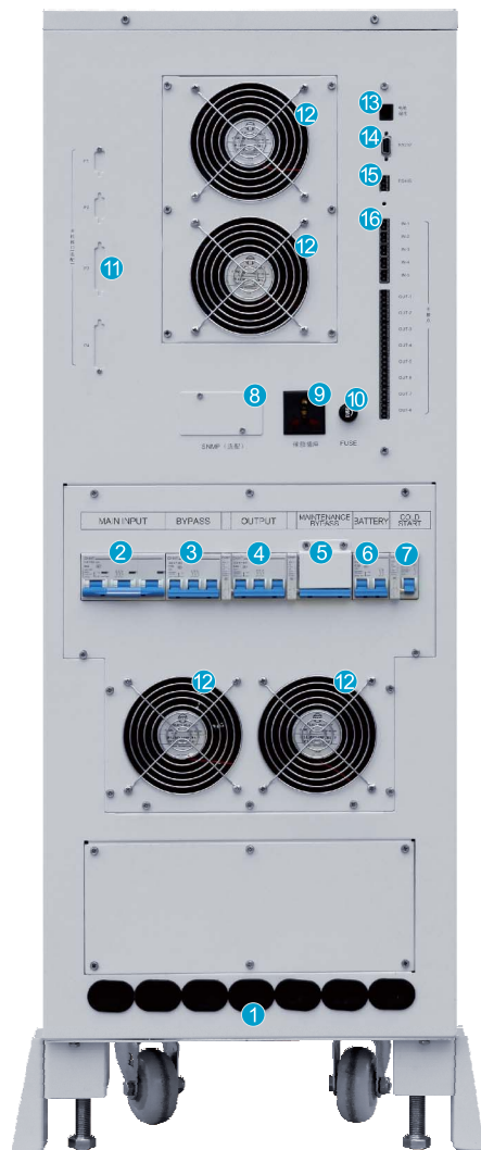
10 – 40KVA Rear panel
